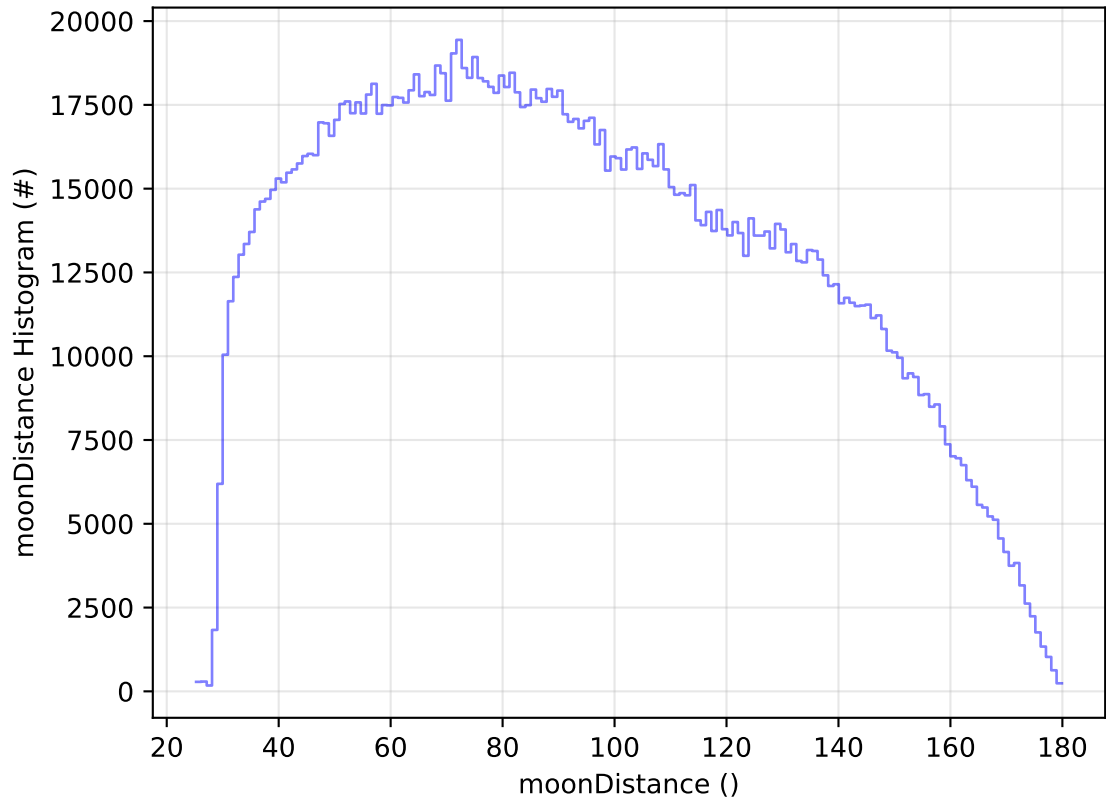
roll_uniform_eh_acc0.2_mjdp0_v3.4_10yrs WFD all bands: moonDistance Histogram
