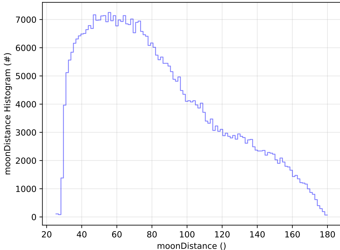
roll_uniform_eh_acc0.2_mjdp0_v3.4_10yrs All sky z band: moonDistance Histogram
