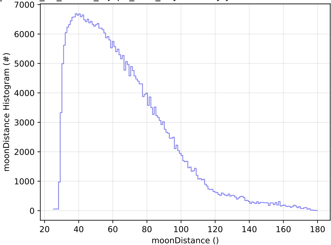
roll_uniform_eh_acc0.2_mjdp0_v3.4_10yrs All sky y band: moonDistance Histogram
