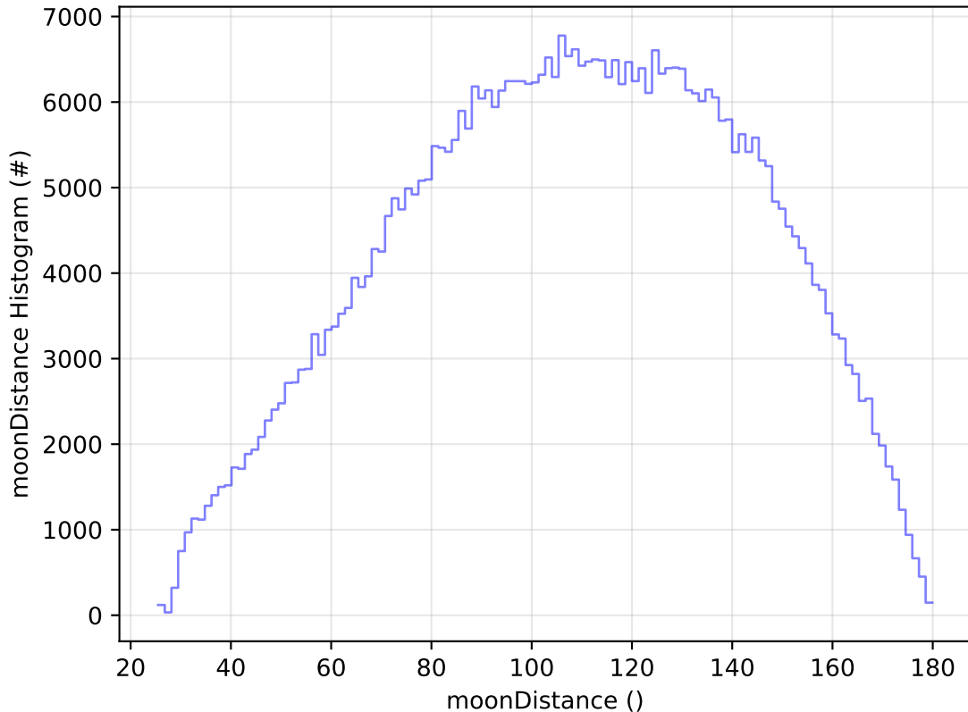
roll_uniform_eh_acc0.2_mjdp0_v3.4_10yrs All sky r band: moonDistance Histogram
