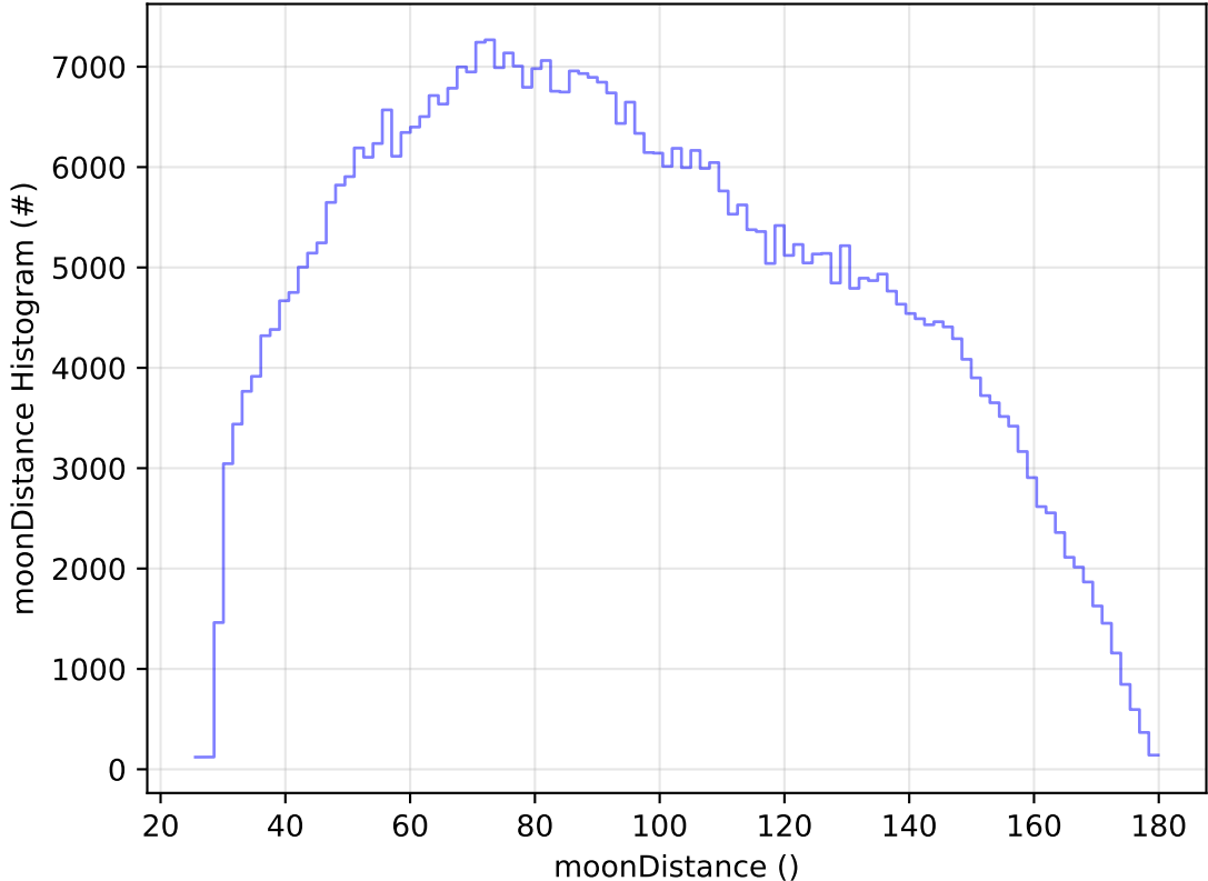
roll_uniform_eh_acc0.2_mjdp0_v3.4_10yrs All sky i band: moonDistance Histogram
