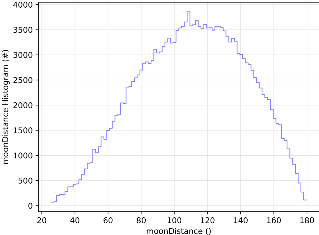
roll_uniform_eh_acc0.2_mjdp0_v3.4_10yrs All sky g band: moonDistance Histogram
