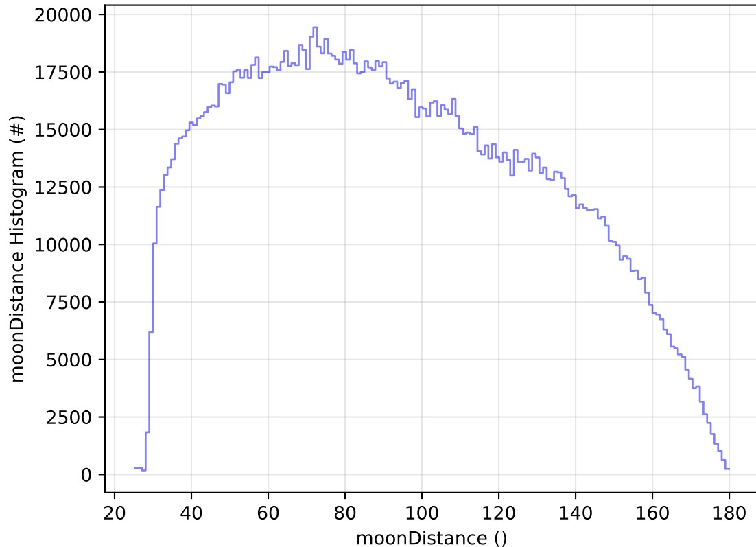
roll_uniform_eh_acc0.2_mjdp0_v3.4_10yrs All sky all bands: moonDistance Histogram
