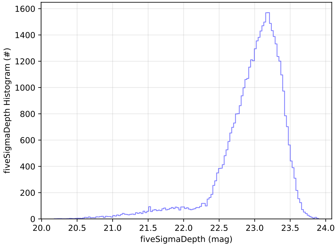
roll_uniform_eh_acc0.2_mjdp0_v3.4_10yrs Yr 1 z band: fiveSigmaDepth Histogram
