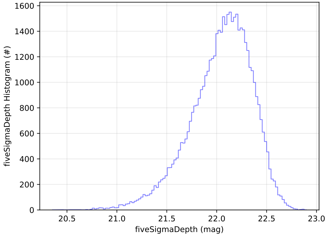
roll_uniform_eh_acc0.2_mjdp0_v3.4_10yrs Yr 1 y band: fiveSigmaDepth Histogram
