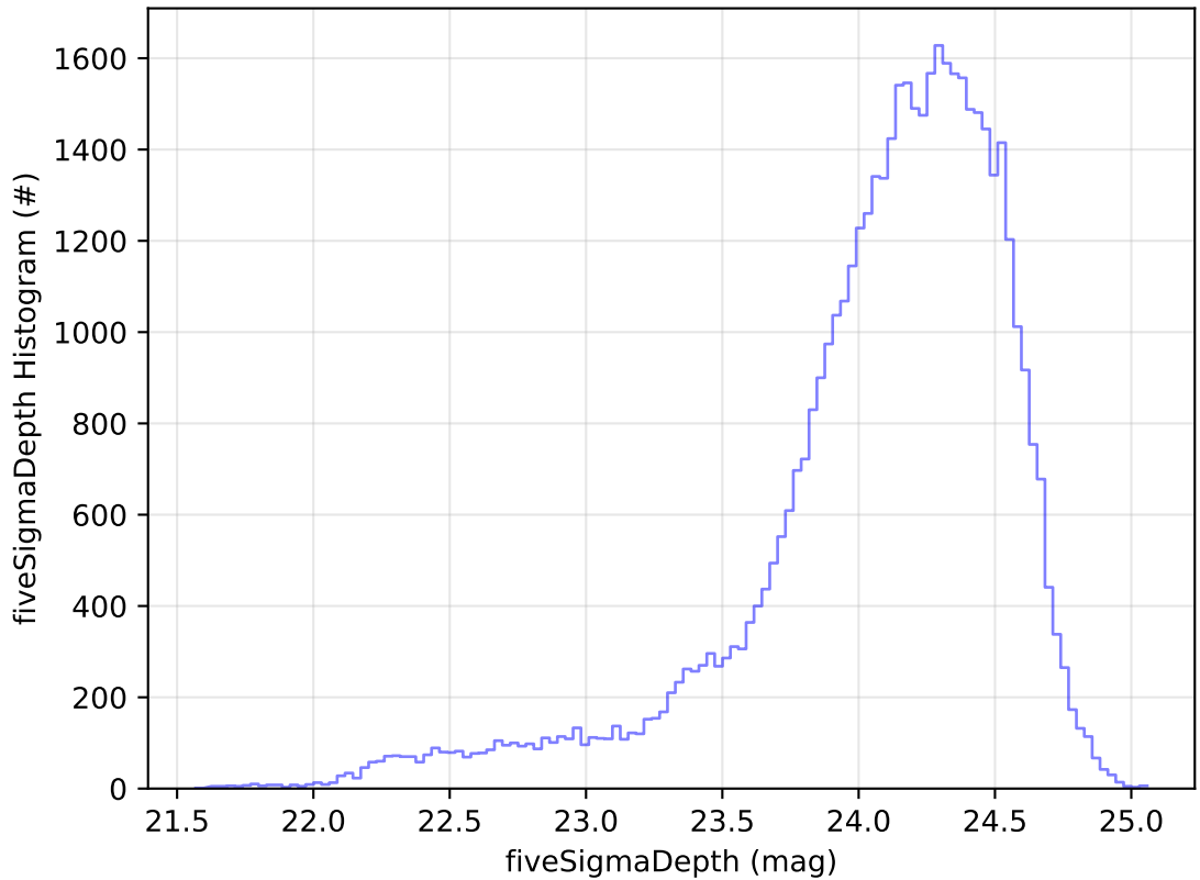
roll_uniform_eh_acc0.2_mjdp0_v3.4_10yrs Yr 1 r band: fiveSigmaDepth Histogram
