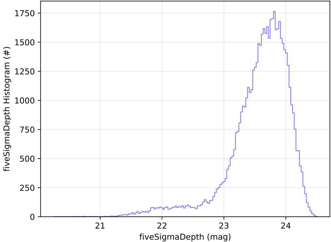
roll_uniform_eh_acc0.2_mjdp0_v3.4_10yrs Yr 1 i band: fiveSigmaDepth Histogram
