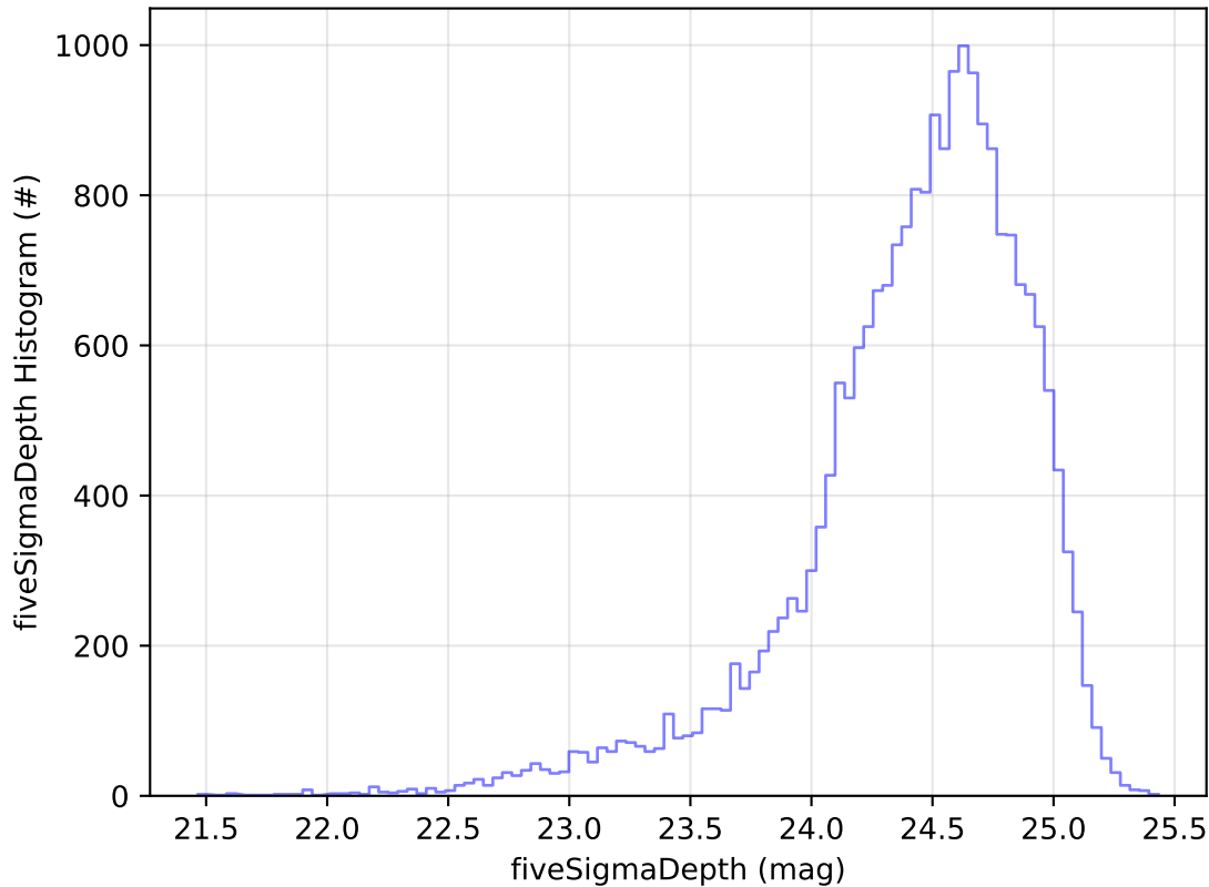
roll_uniform_eh_acc0.2_mjdp0_v3.4_10yrs Yr 1 g band: fiveSigmaDepth Histogram
