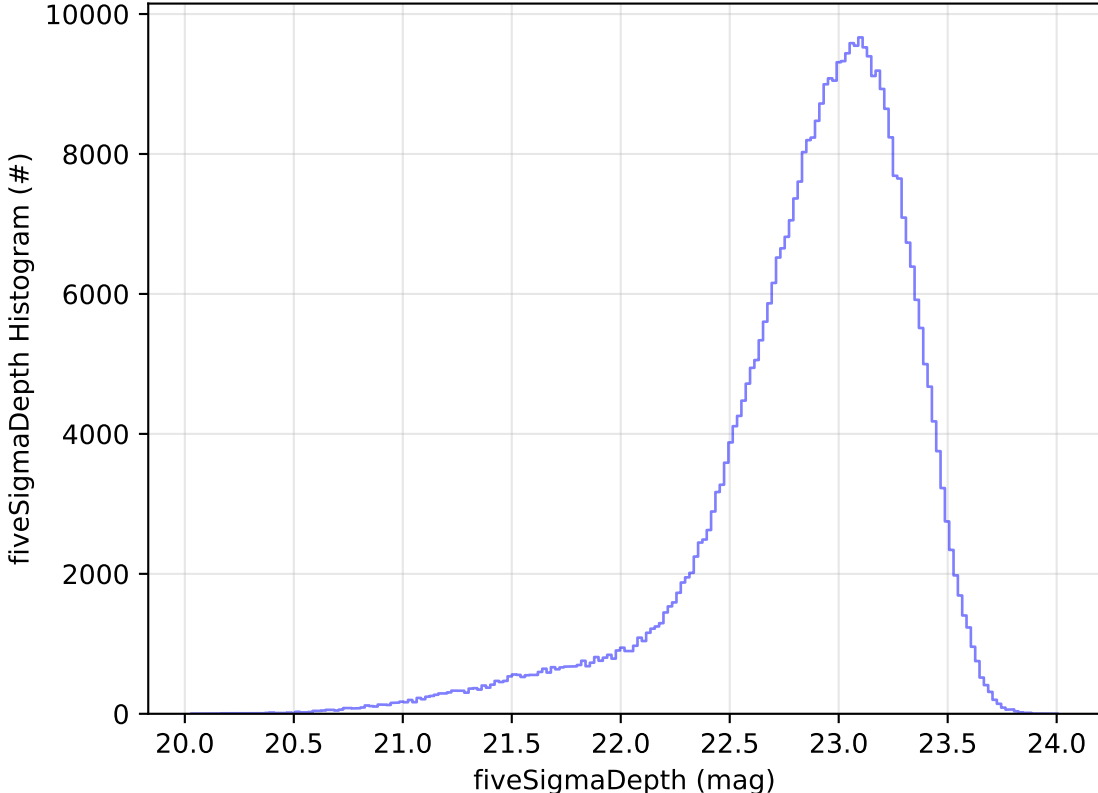
roll_uniform_eh_acc0.2_mjdp0_v3.4_10yrs WFD z band: fiveSigmaDepth Histogram
