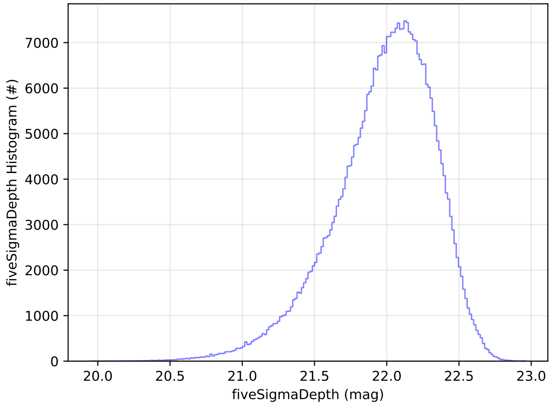
roll_uniform_eh_acc0.2_mjdp0_v3.4_10yrs WFD y band: fiveSigmaDepth Histogram
