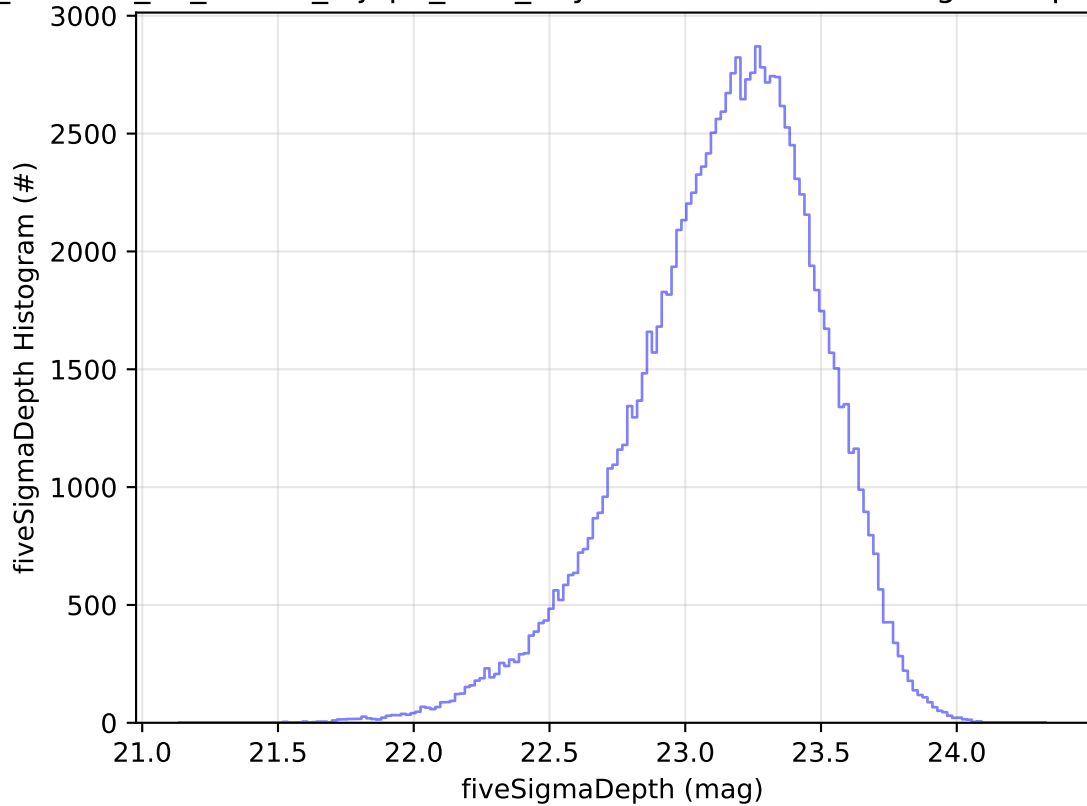
roll_uniform_eh_acc0.2_mjdp0_v3.4_10yrs WFD u band: fiveSigmaDepth Histogram
