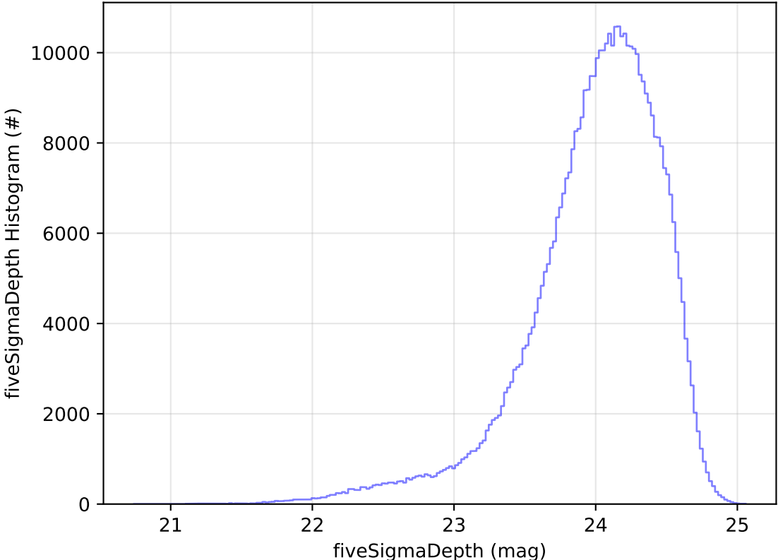
roll_uniform_eh_acc0.2_mjdp0_v3.4_10yrs WFD r band: fiveSigmaDepth Histogram
