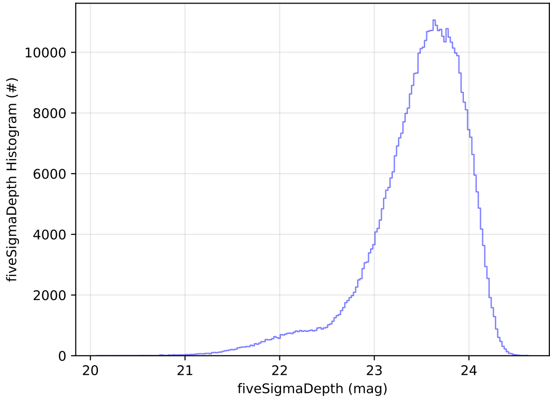
roll_uniform_eh_acc0.2_mjdp0_v3.4_10yrs WFD i band: fiveSigmaDepth Histogram
