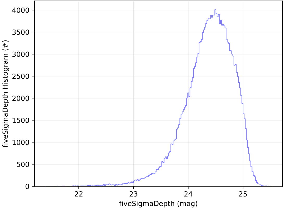
roll_uniform_eh_acc0.2_mjdp0_v3.4_10yrs WFD g band: fiveSigmaDepth Histogram
