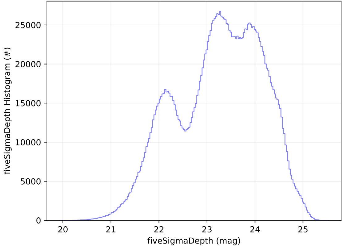
roll_uniform_eh_acc0.2_mjdp0_v3.4_10yrs WFD all bands: fiveSigmaDepth Histogram
