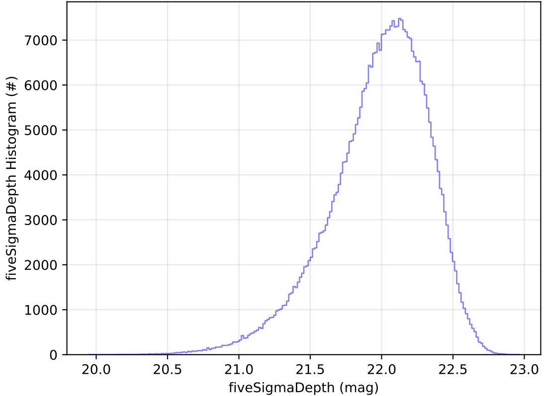
roll_uniform_eh_acc0.2_mjdp0_v3.4_10yrs All sky y band: fiveSigmaDepth Histogram
