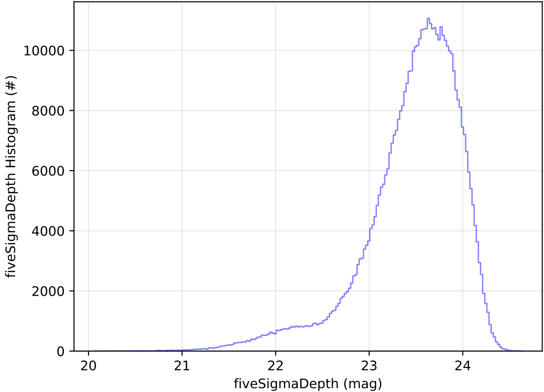
roll_uniform_eh_acc0.2_mjdp0_v3.4_10yrs All sky i band: fiveSigmaDepth Histogram
