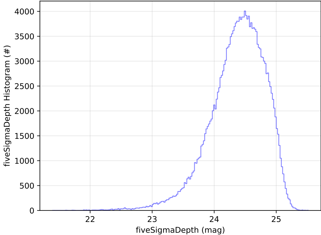
roll_uniform_eh_acc0.2_mjdp0_v3.4_10yrs All sky g band: fiveSigmaDepth Histogram
