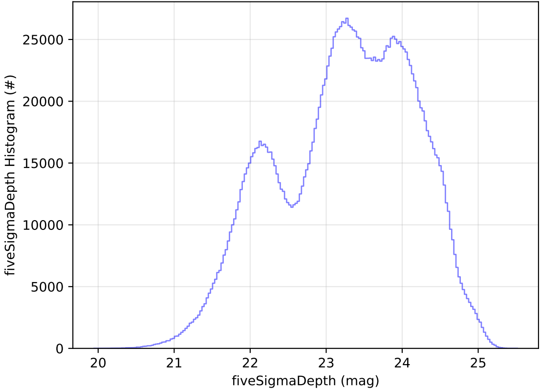
roll_uniform_eh_acc0.2_mjdp0_v3.4_10yrs All sky all bands: fiveSigmaDepth Histogram
