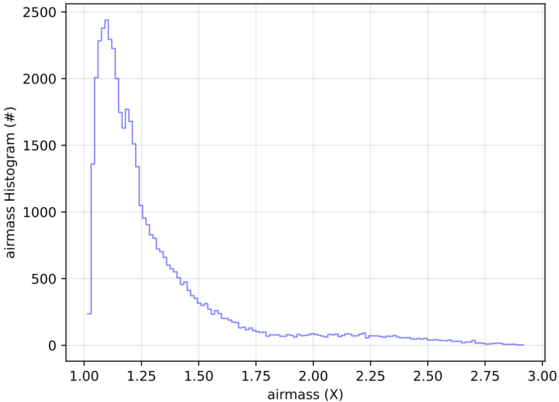
roll_uniform_eh_acc0.2_mjdp0_v3.4_10yrs Yr 1 z band: airmass Histogram
