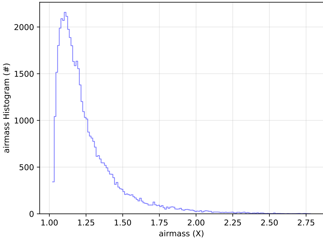
roll_uniform_eh_acc0.2_mjdp0_v3.4_10yrs Yr 1 y band: airmass Histogram
