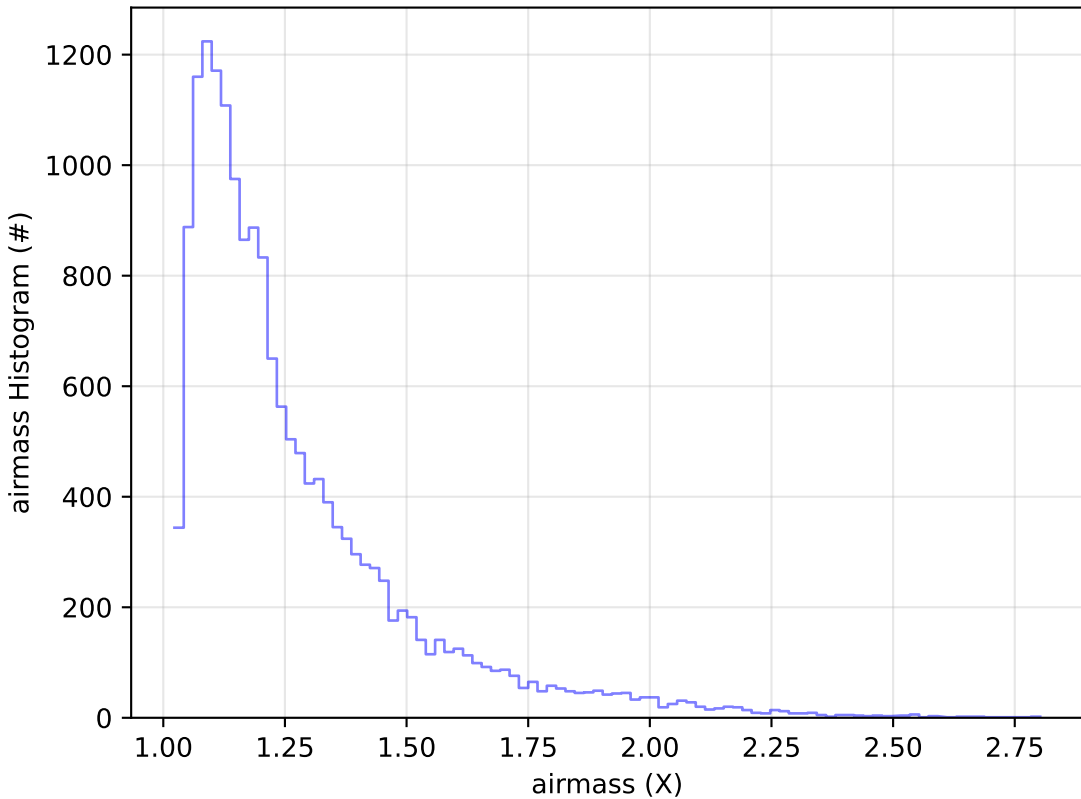
roll_uniform_eh_acc0.2_mjdp0_v3.4_10yrs Yr 1 u band: airmass Histogram
