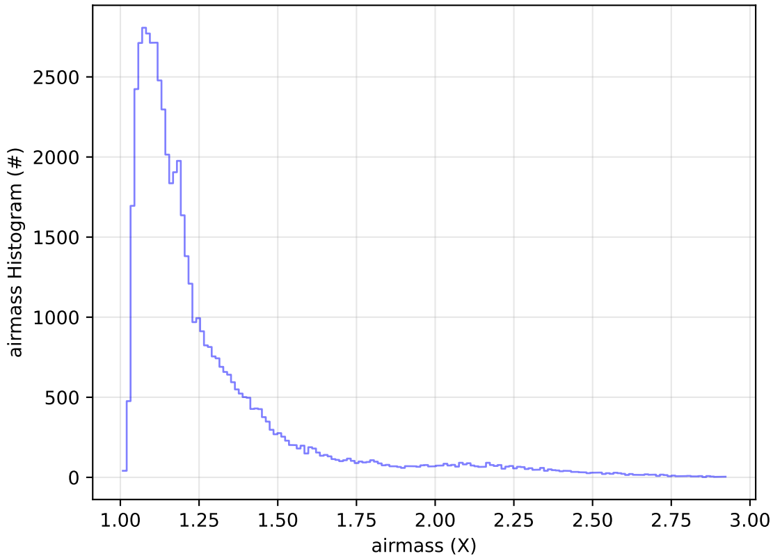
roll_uniform_eh_acc0.2_mjdp0_v3.4_10yrs Yr 1 i band: airmass Histogram
