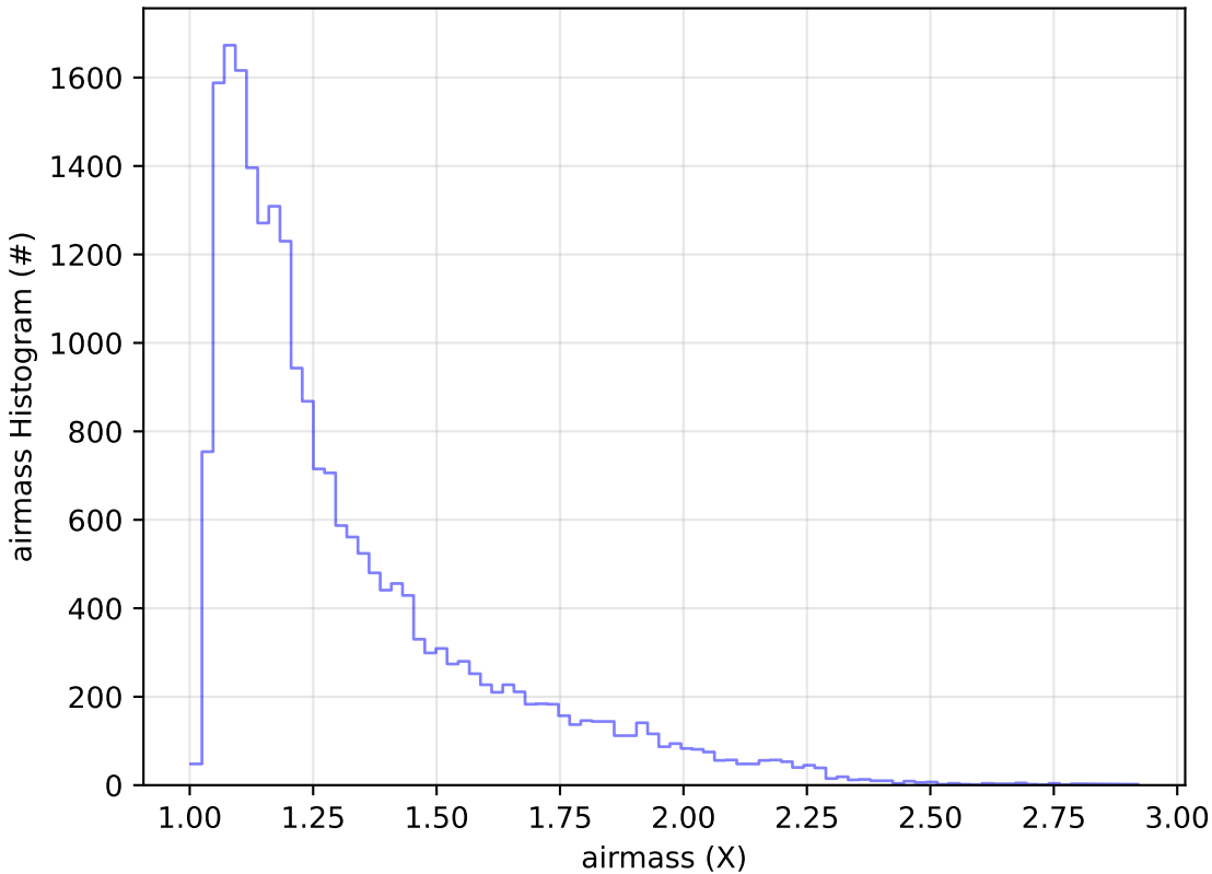
roll_uniform_eh_acc0.2_mjdp0_v3.4_10yrs Yr 1 g band: airmass Histogram
