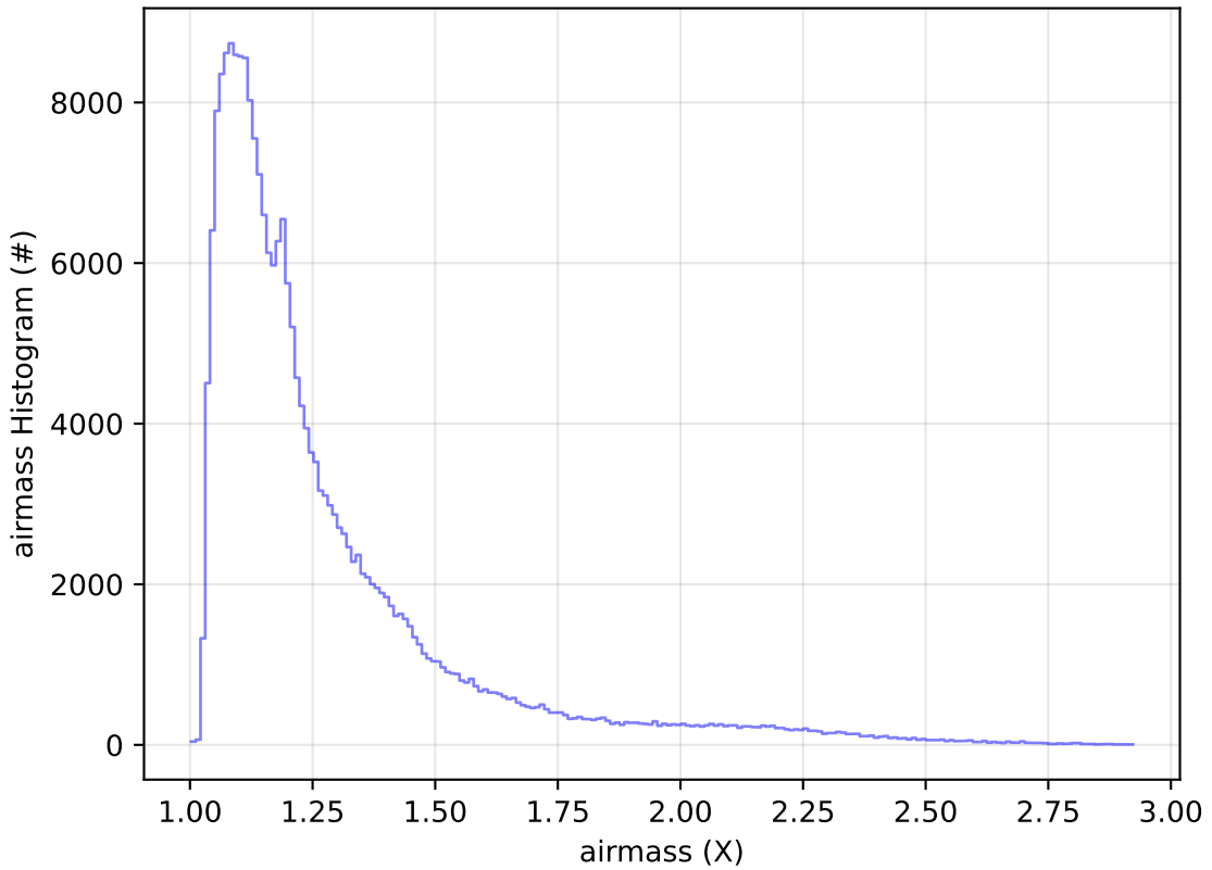
roll_uniform_eh_acc0.2_mjdp0_v3.4_10yrs Yr 1 all bands: airmass Histogram
