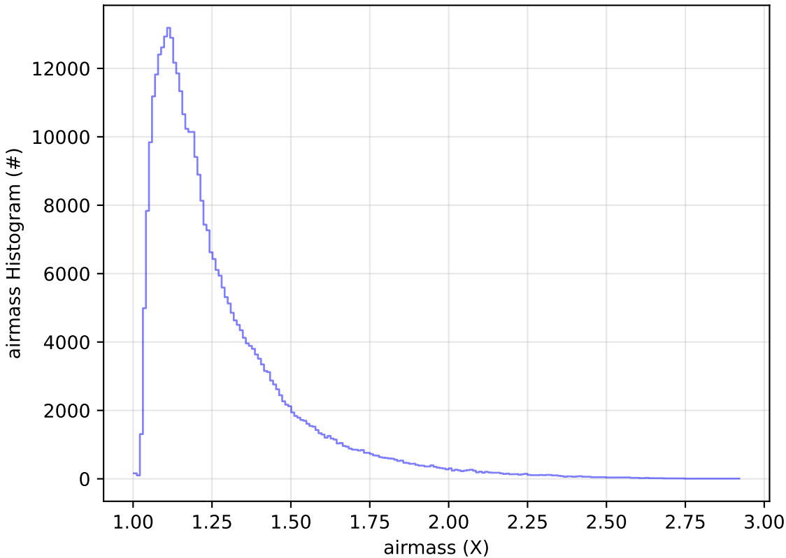
roll_uniform_eh_acc0.2_mjdp0_v3.4_10yrs WFD y band: airmass Histogram
