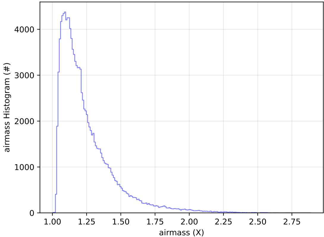
roll_uniform_eh_acc0.2_mjdp0_v3.4_10yrs WFD u band: airmass Histogram
