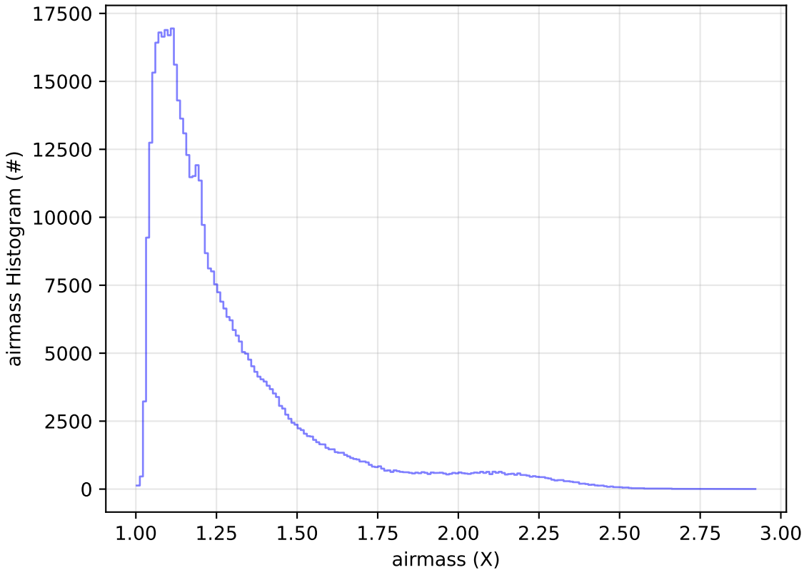
roll_uniform_eh_acc0.2_mjdp0_v3.4_10yrs WFD r band: airmass Histogram
