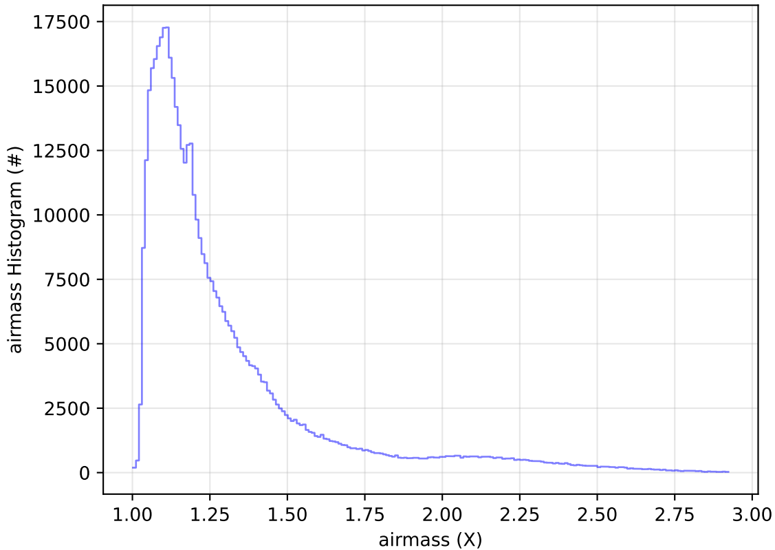
roll_uniform_eh_acc0.2_mjdp0_v3.4_10yrs WFD i band: airmass Histogram
