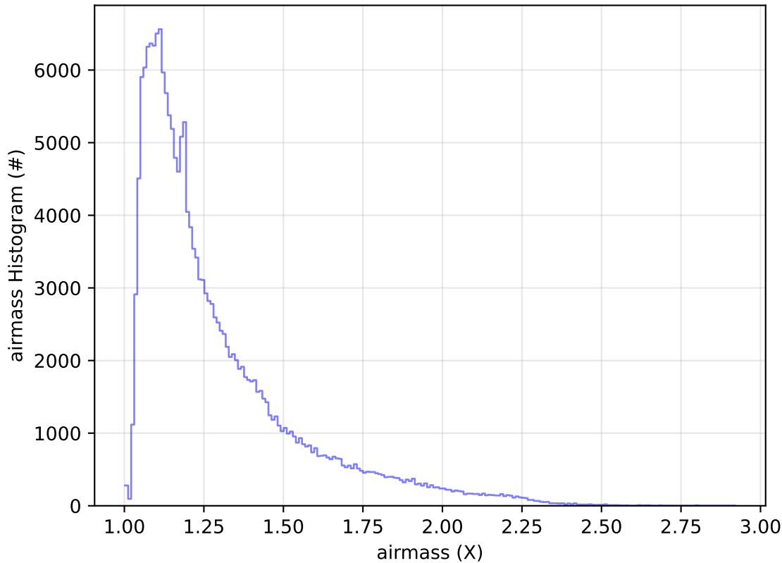
roll_uniform_eh_acc0.2_mjdp0_v3.4_10yrs WFD g band: airmass Histogram
