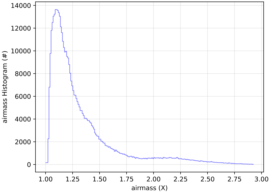
roll_uniform_eh_acc0.2_mjdp0_v3.4_10yrs All sky z band: airmass Histogram
