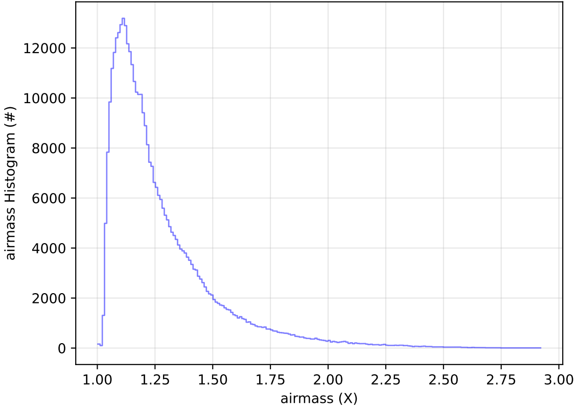
roll_uniform_eh_acc0.2_mjdp0_v3.4_10yrs All sky y band: airmass Histogram
