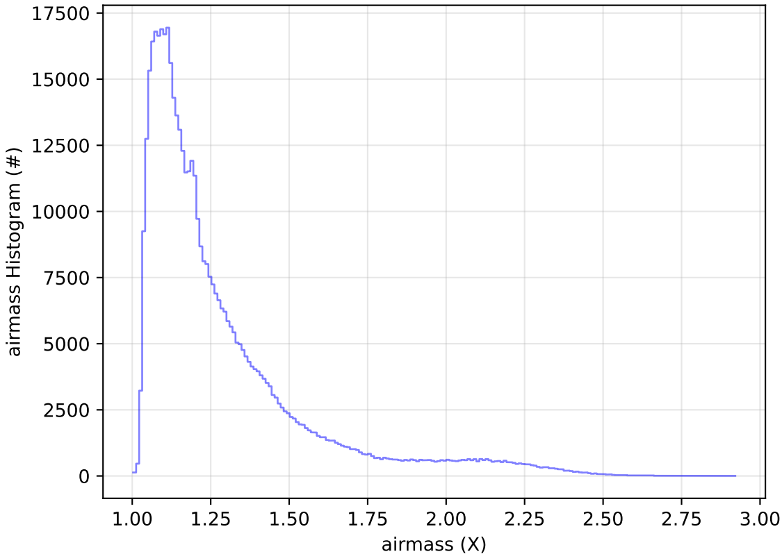
roll_uniform_eh_acc0.2_mjdp0_v3.4_10yrs All sky r band: airmass Histogram
