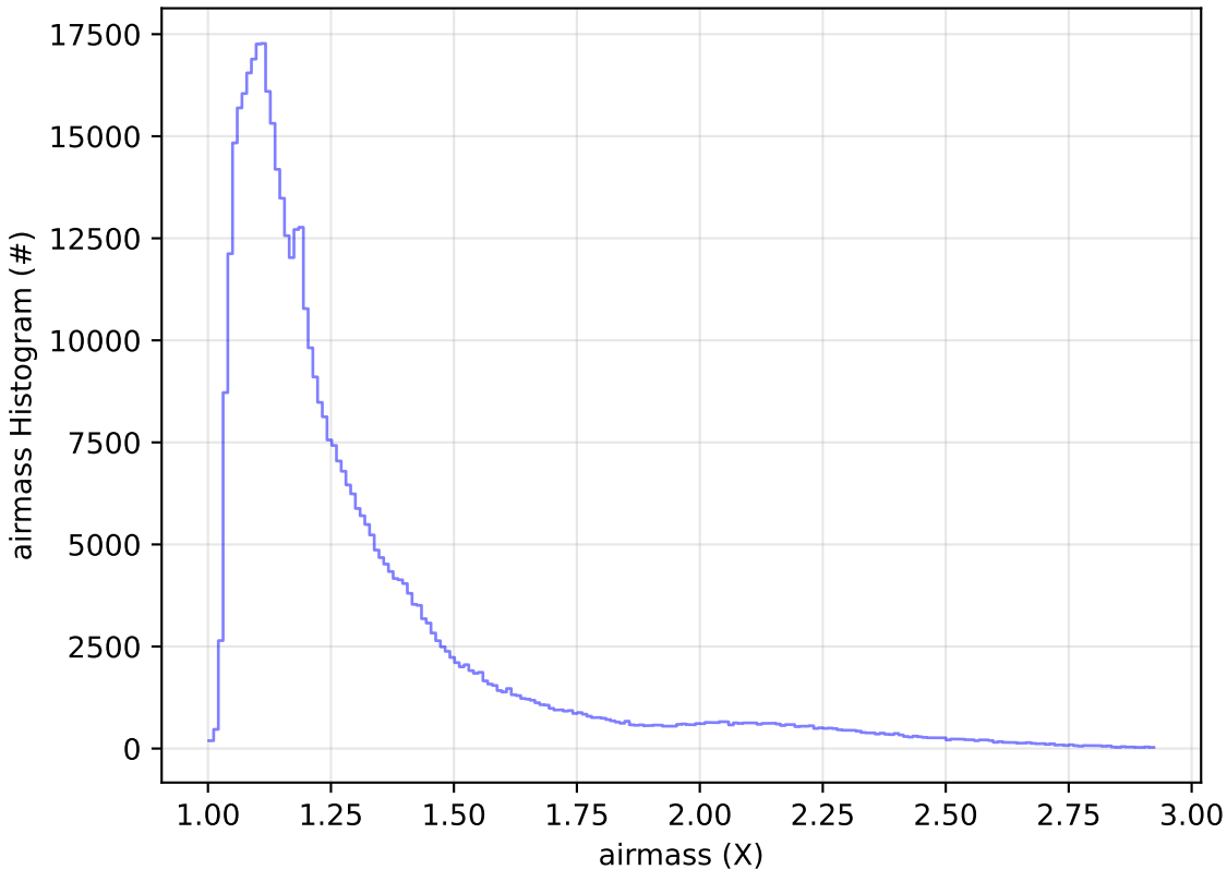
roll_uniform_eh_acc0.2_mjdp0_v3.4_10yrs All sky i band: airmass Histogram
