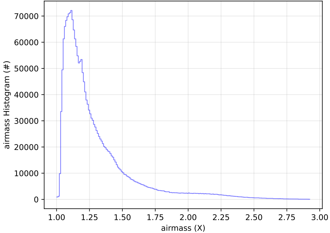
roll_uniform_eh_acc0.2_mjdp0_v3.4_10yrs All sky all bands: airmass Histogram
