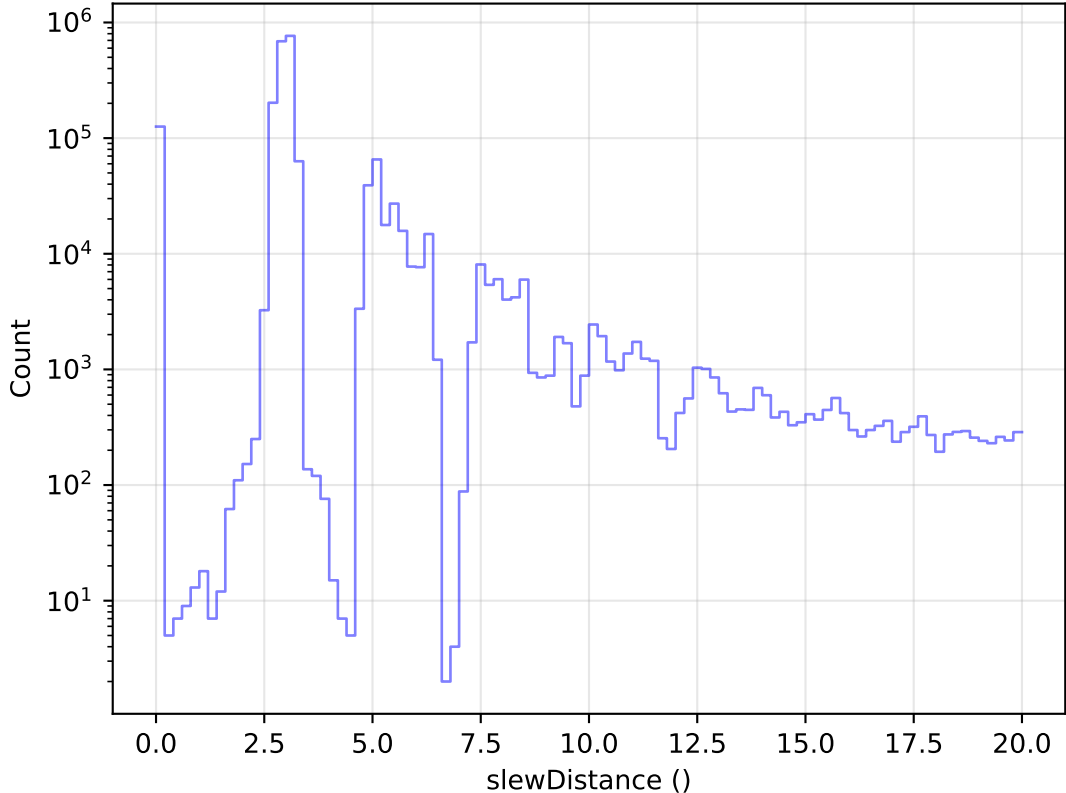
roll_uniform_eh_acc0.2_mjdp0_v3.4_10yrs All visits: Zoom Slew Distance Histogram
