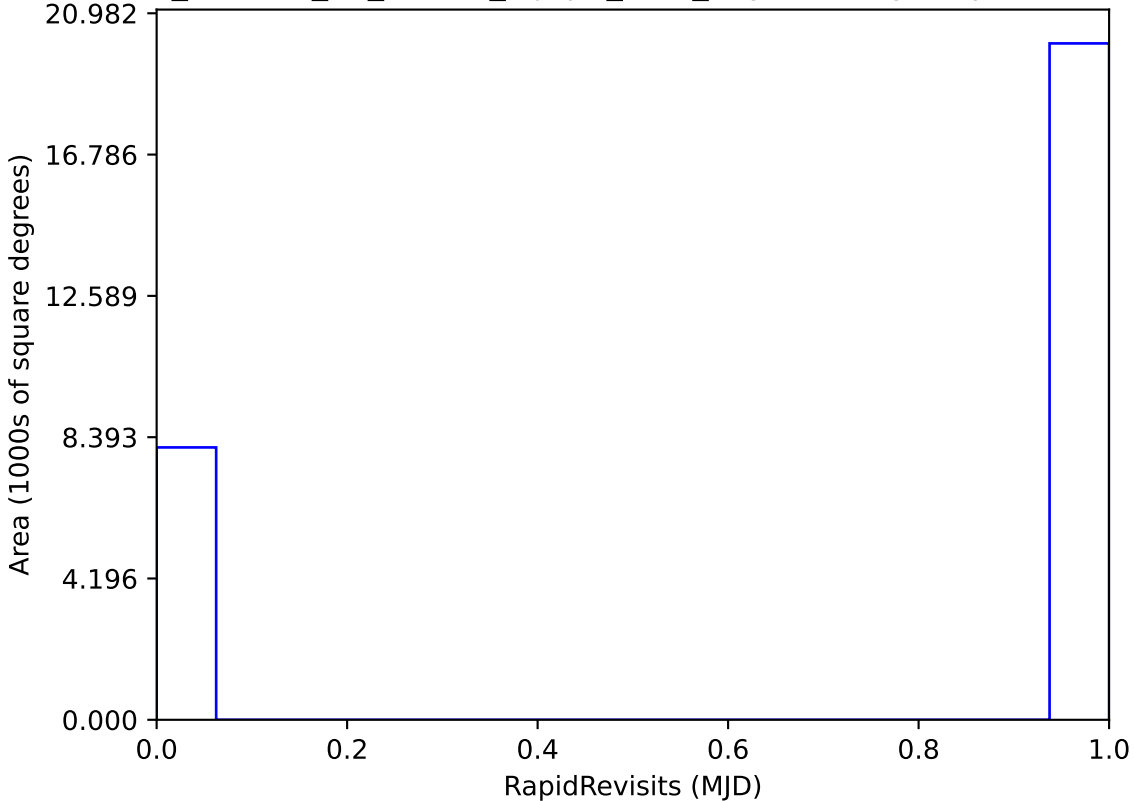
roll_uniform_eh_acc0.2_mjdp0_v3.4_10yrs All sky: RapidRevisits
