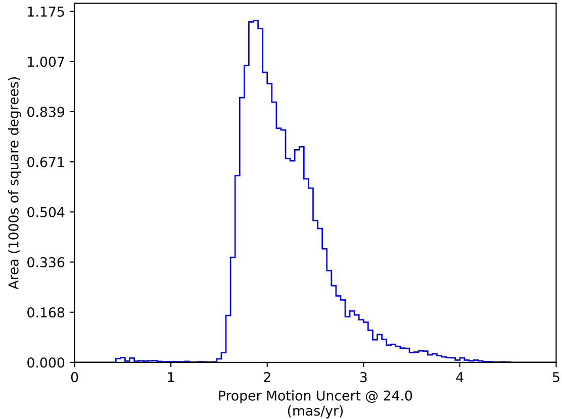
roll_uniform_eh_acc0.2_mjdp0_v3.4_10yrs WFD: Proper Motion Uncert @ 24.0
