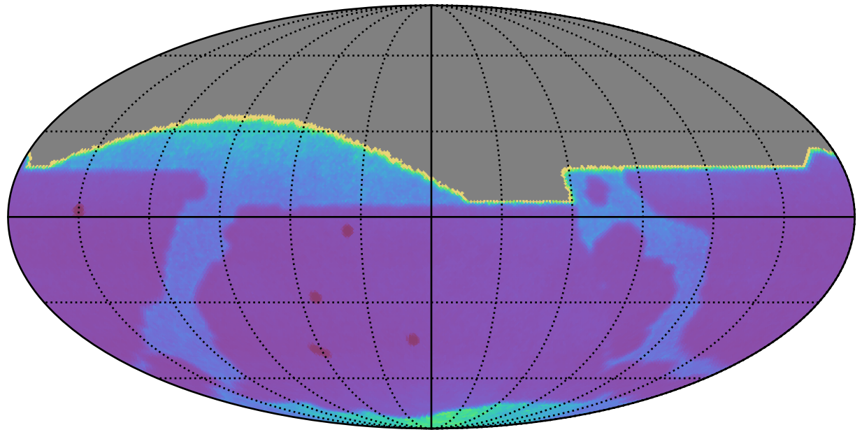
roll_uniform_eh_acc0.2_mjdp0_v3.4_10yrs All sky: Proper Motion Uncert @ 20.5
