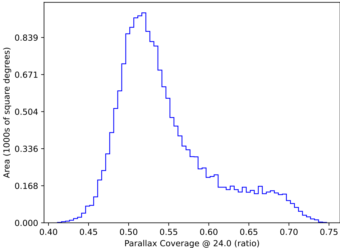
roll_uniform_eh_acc0.2_mjdp0_v3.4_10yrs WFD: Parallax Coverage @ 24.0
