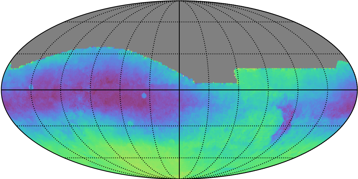
roll_uniform_eh_acc0.2_mjdp0_v3.4_10yrs All sky: Parallax-DCR degeneracy @ 24.0
