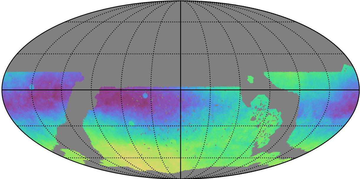
roll_uniform_eh_acc0.2_mjdp0_v3.4_10yrs WFD: Parallax-DCR degeneracy @ 22.4
