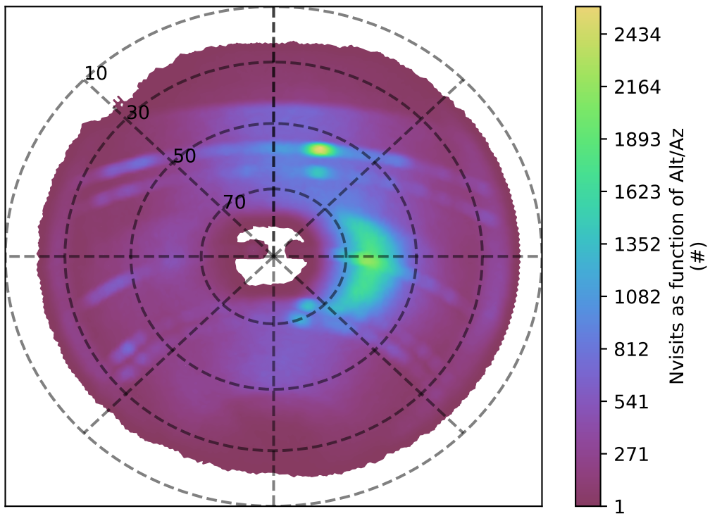
roll_uniform_eh_acc0.2_mjdp0_v3.4_10yrs z band: Nvisits as function of Alt/Az
