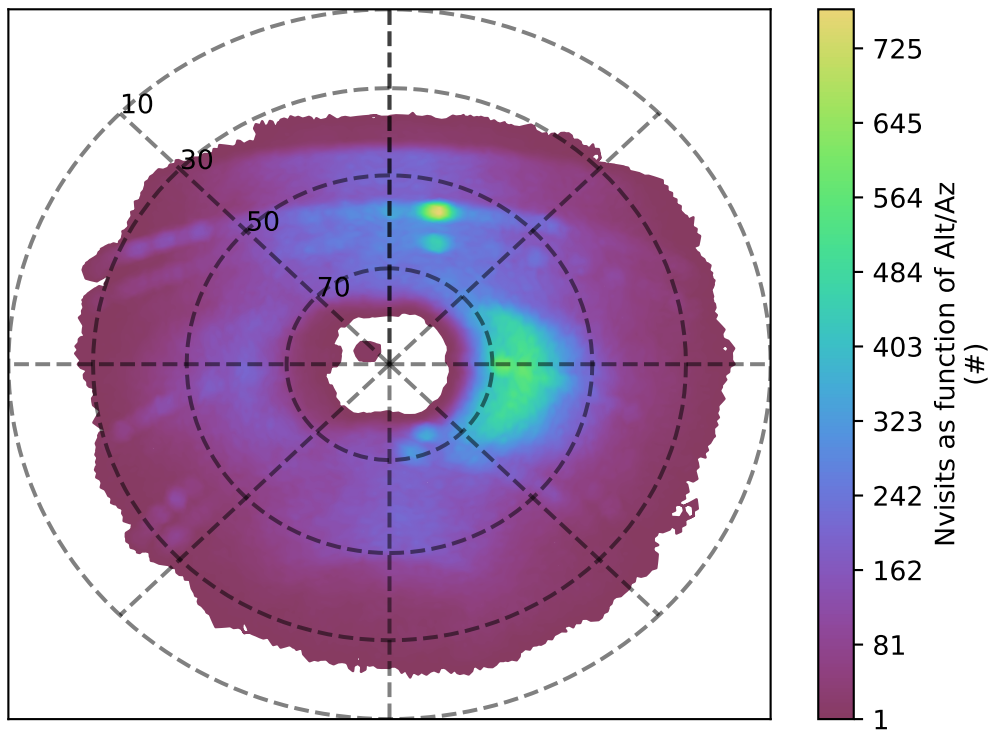
roll_uniform_eh_acc0.2_mjdp0_v3.4_10yrs u band: Nvisits as function of Alt/Az
