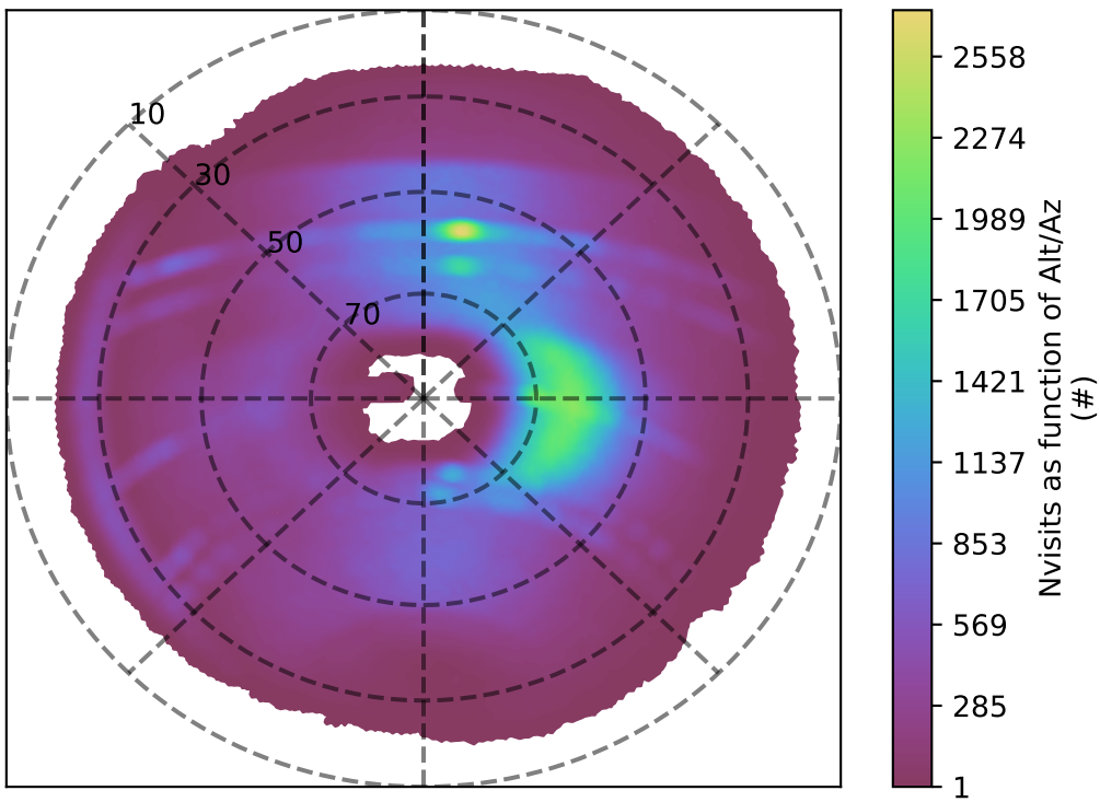
roll_uniform_eh_acc0.2_mjdp0_v3.4_10yrs r band: Nvisits as function of Alt/Az
