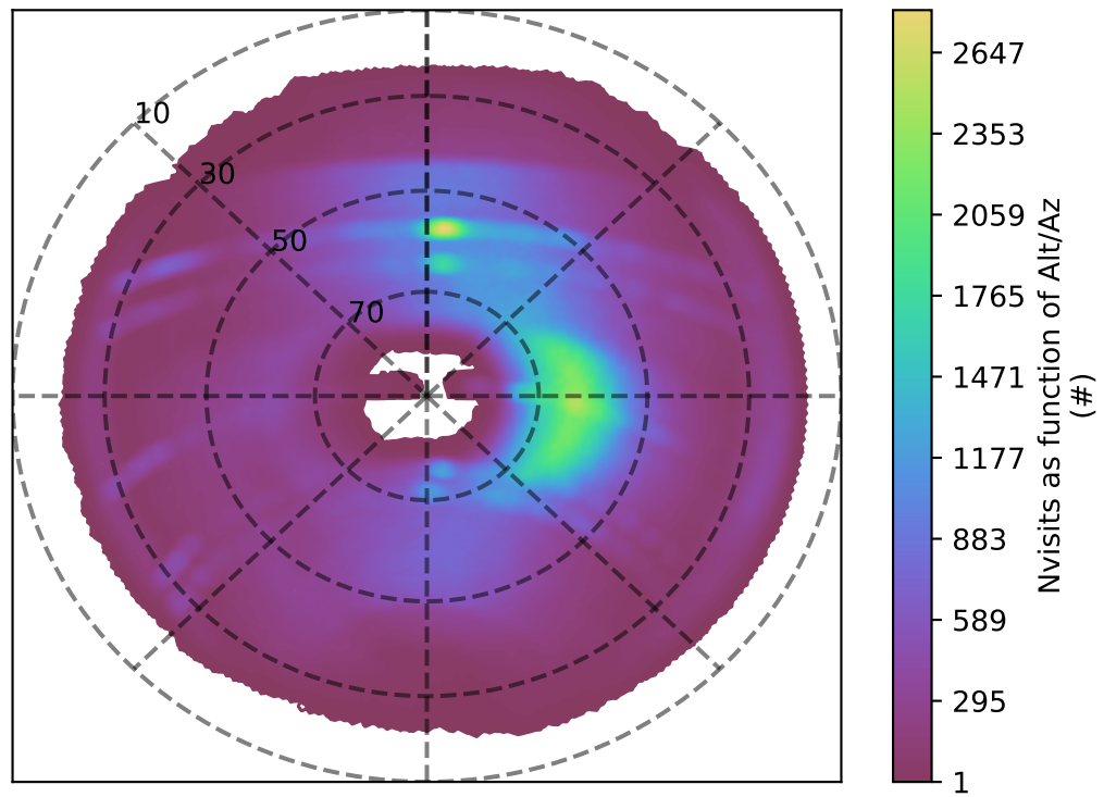
roll_uniform_eh_acc0.2_mjdp0_v3.4_10yrs i band: Nvisits as function of Alt/Az
